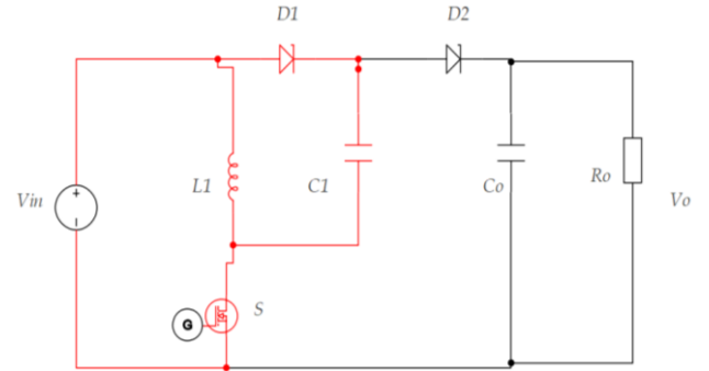
Fig 3(a). when Switch S is ON
