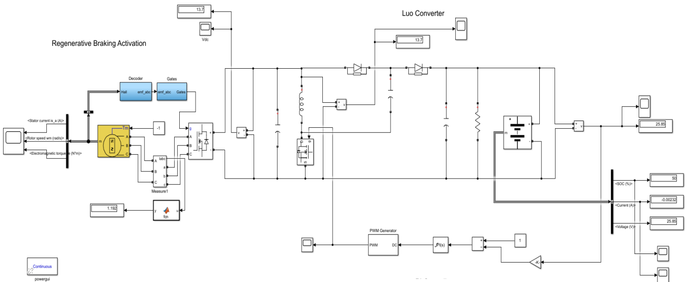
Fig 4. Simulation of proposed Luo converter Integration.
