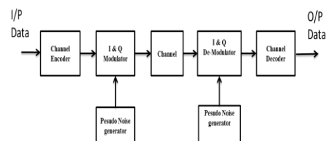
Figure 1: Block diagram of Spread Spectrum Communication system
