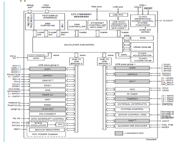
Figure 8: Block diagram of ARM CORTEX M3 Controller
