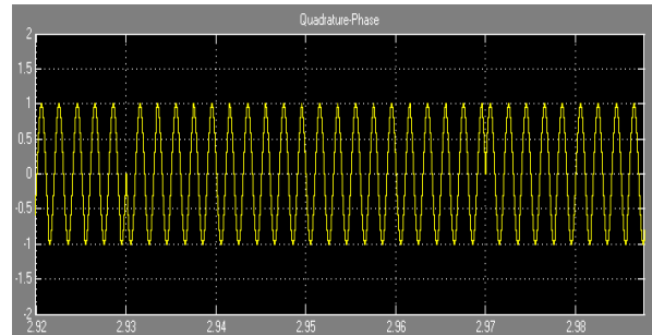
Figure 16: Quadrature phase modulation signal
