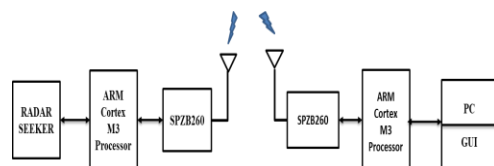
Figure 6: Block diagram of CDMA TransReceiver system
