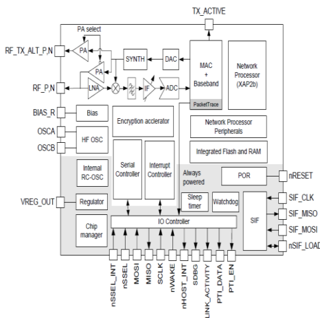
Figure 7: Block diagram of SPZB260
