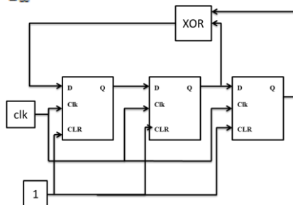
Figure 3: Block diagram of Pseudo Random generator
