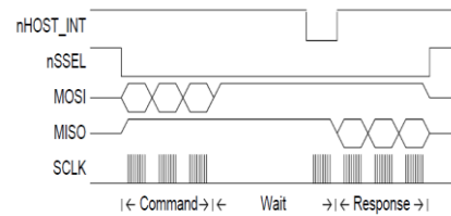
Figure 9: SPI transaction between microcontroller and SPZB260
