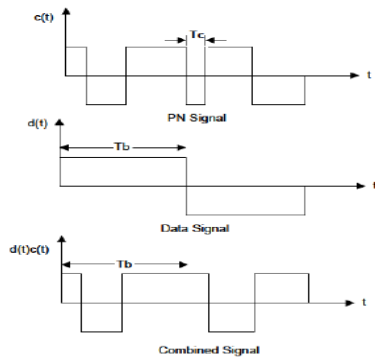
Figure 2: Wave form of Pseudo Random generator
