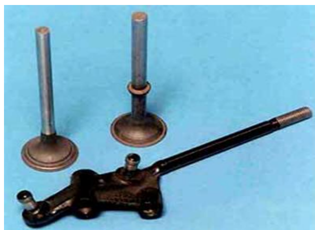
Fig. 6 Friction welded automotive components (Engine valves and tie rod)
