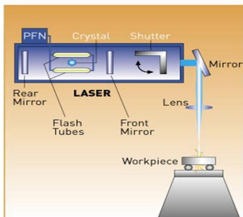
Fig. 7 Diagram of laser beam welding (Source: Oguzhan Yılmaz )
