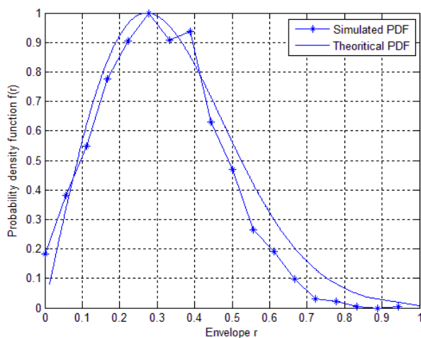
Fig: 3 Probability density function of Rayleigh fading channel
