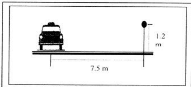
Fig.6 Location of the sound level meter
