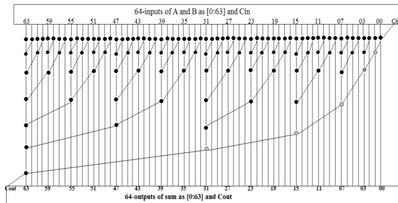
Fig3: proposed 64-bit parallel prefix adder
