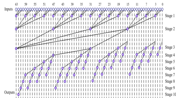
Fig2: existed 64-bit parallel prefix adder
