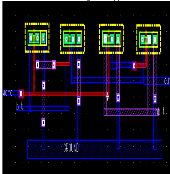
Fig 9: 4T CAM Cell layout in 0.18 um standard CMOS Technology.
