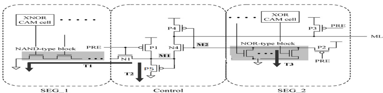
Fig 7: HYBRID CAM Structure [Ref 7]
