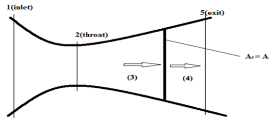
Fig.2.2.1 Convergent divergent nozzle
