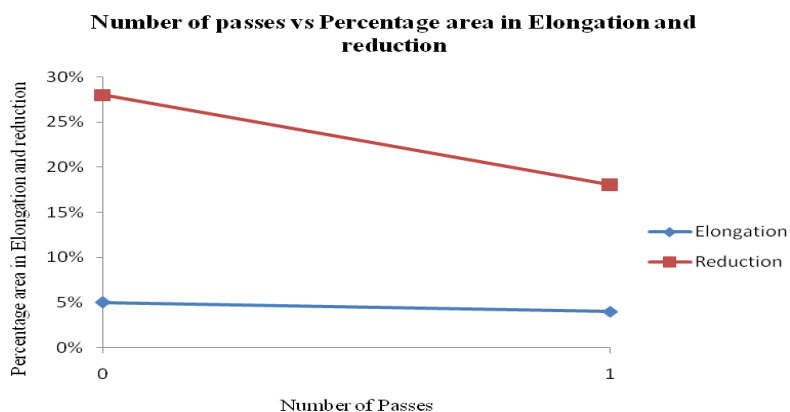
Fig. 3.2 Number of Passes Vs Percentage area in Elongation and reduction
