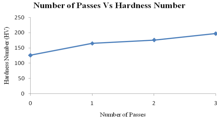
Fig 3.3 Number of passes vs Hardness number
