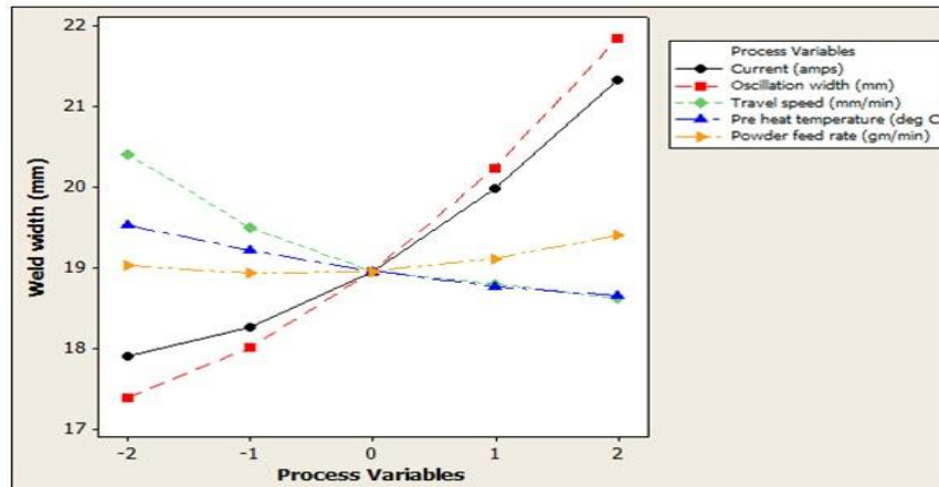
Figure 4: Direct effect of process variables on weld with
