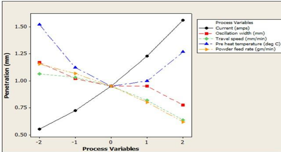
Figure 2: Direct effect of process variables on penetration
