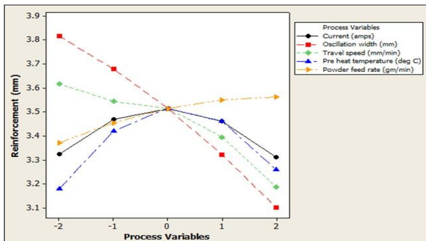
Figure 3: Direct effect of process variables on reinforcement
