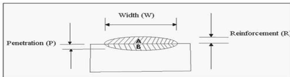
Figure 1: Weld bead geometry
