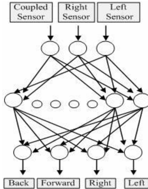
Figure 3. Neural Network Model
