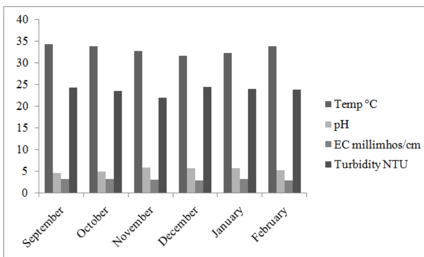
Fig. 3.1: Seasonal variation of physical parameters in paper mill effluent
